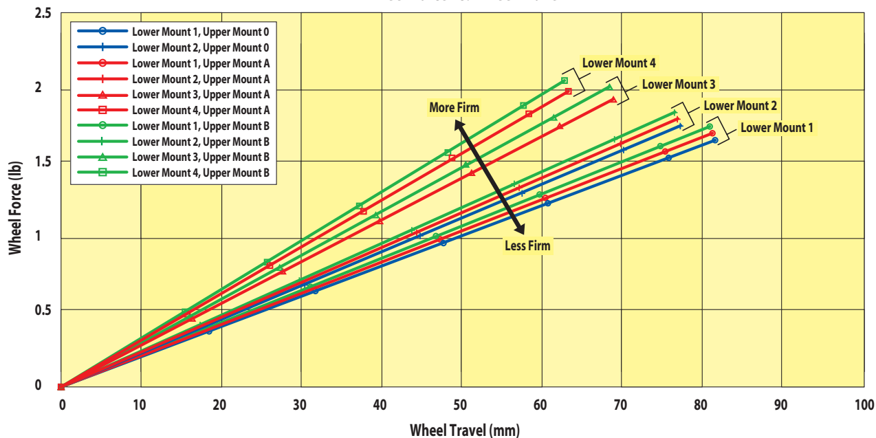
Wheel Force vs. Wheel Travel
